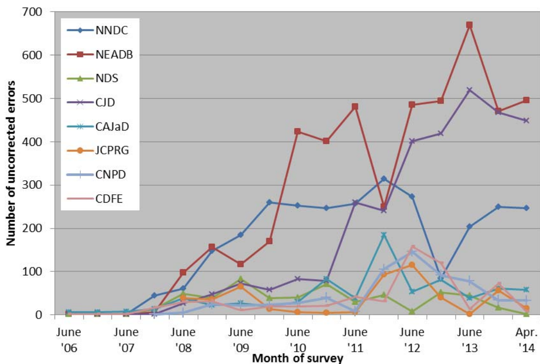
Fig.1: Time evolution of the total number of uncorrected errors in the feedback list. Errors corrected but not included in the EXFOR Master (~480 for NEA DB, ~30 for CJD and CNPD) are not taken into account.
