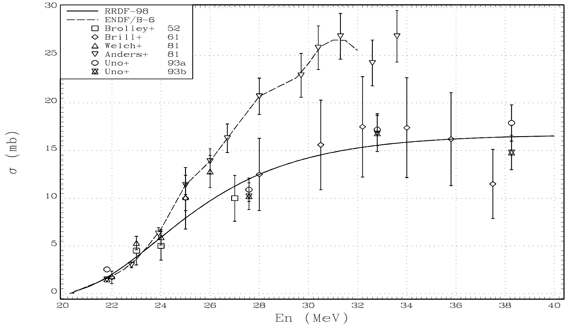
Fig.1. RRDF-98 evaluated excitation function for the ^{12}\text{C}(n,2n)^{11}\text{C} reaction in comparison with ENDF/B-VI curve and experimental data.
