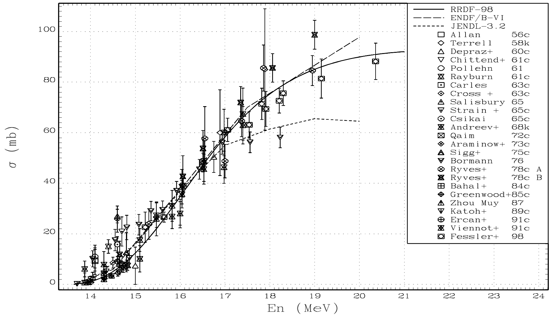
Fig.12. RRDF-98 evaluated excitation function for the ^{54}\text{Fe}(n,2n)^{53\text{m}+\text{g}}\text{Fe} reaction in comparison with ENDF/B-VI and JENDL-3.2 curves and experimental data.
