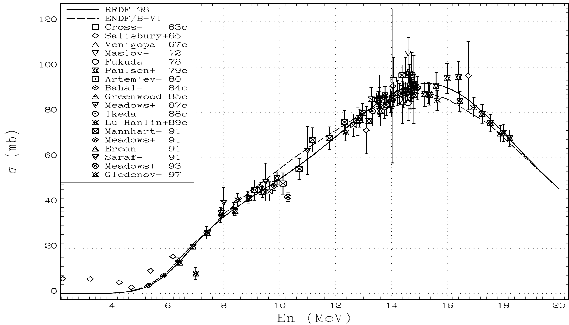
Fig.13. RRDF-98 evaluated excitation function for the ^{54}\text{Fe}(n,\alpha)^{51}\text{Cr} reaction in comparison with ENDF/B-VI curve and experimental data.
