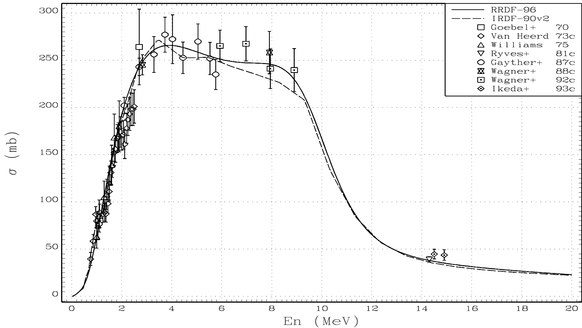
Fig.19. RRDF-98 evaluated excitation function for the ^{93}\text{Nb}(n,n')^{93\text{m}}\text{Nb} reaction in comparison with IRDF-90 (version 2) curve and experimental data.
