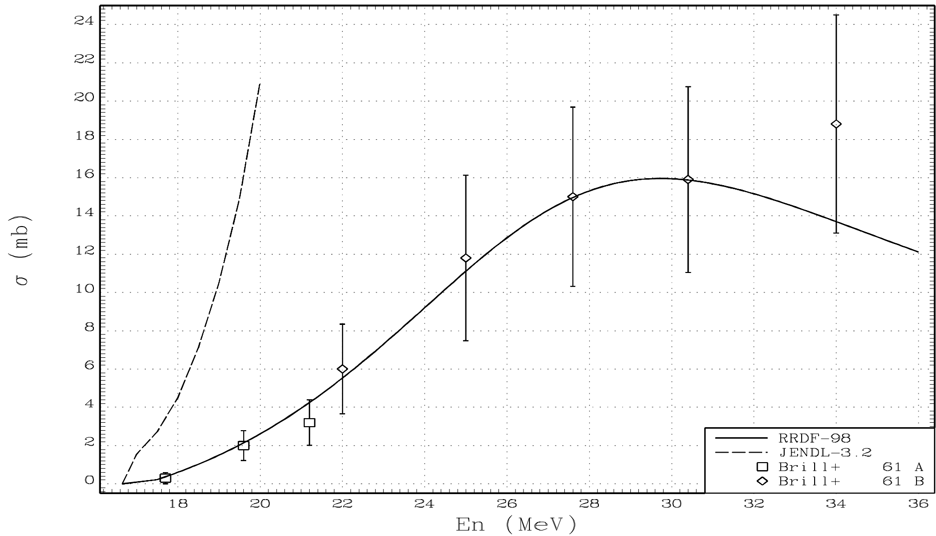
Fig.2. RRDF-98 evaluated excitation function for the ^{16}\text{O}(n,2n)^{15}\text{O} reaction in comparison with JENDL-3.2 curve and experimental data.
