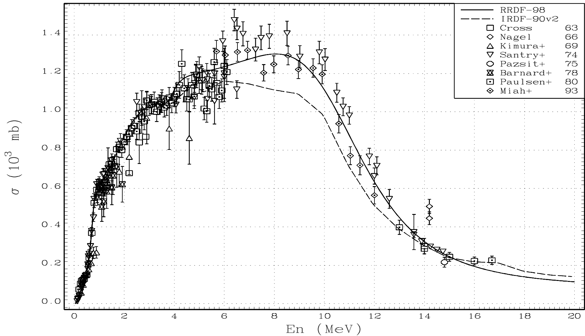
Fig.20. RRDF-98 evaluated excitation function for the ^{103}\text{Rh}(n,n')^{103\text{m}}\text{Rh} reaction in comparison with IRDF-90 (version 2) curve and experimental data.
