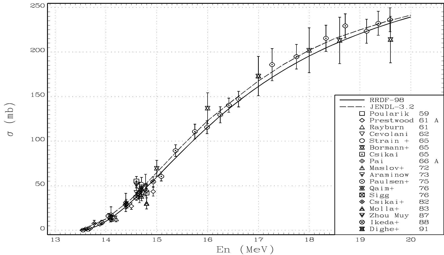
Fig.5. RRDF-98 evaluated excitation function for the ^{46}\text{Ti}(n,2n)^{45}\text{Ti} reaction in comparison with JENDL-3.2 curve and experimental data.
