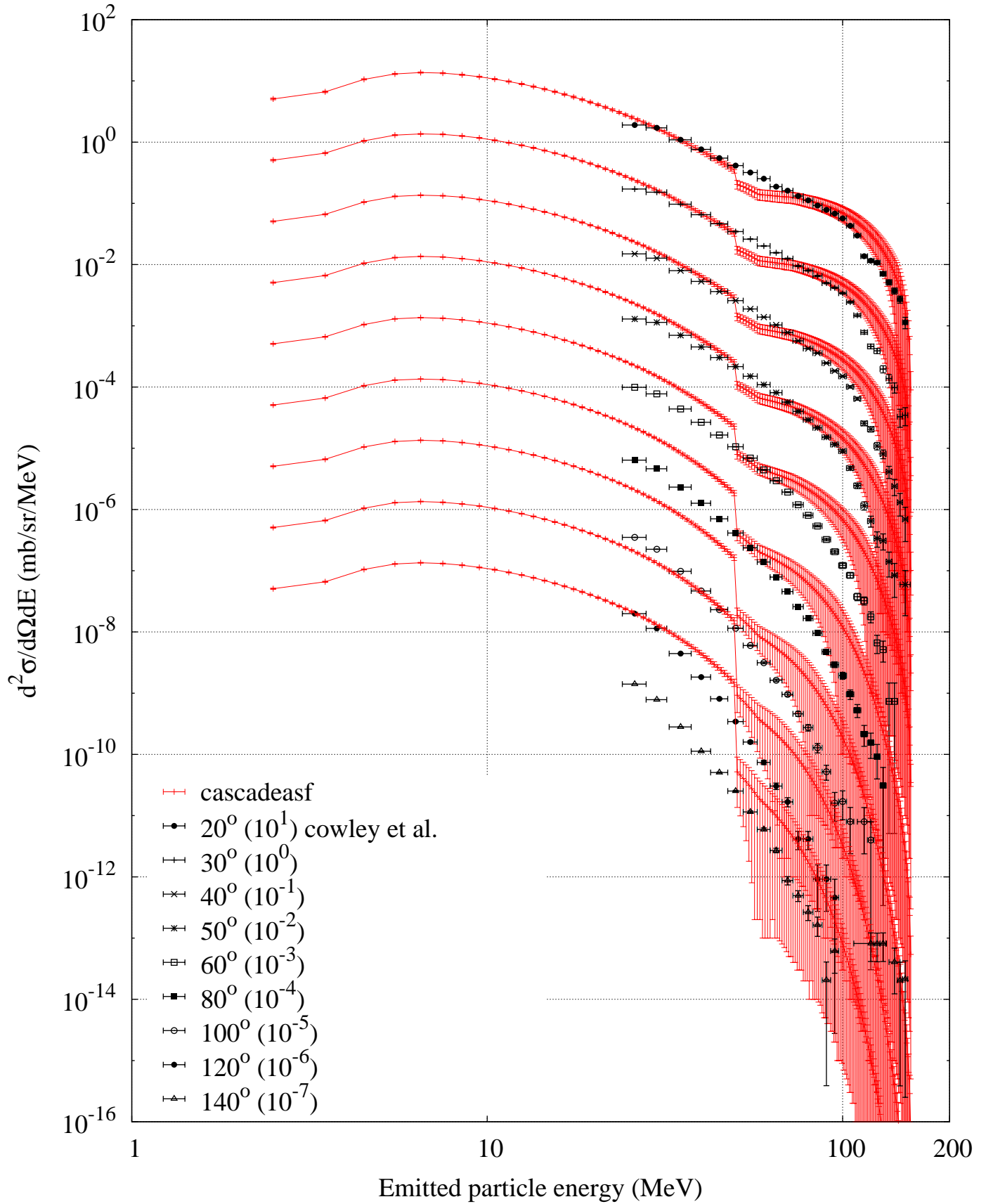
p (160 MeV) + Al -- Helium-4 spectrum
