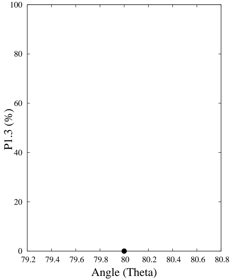
P1.3 factor - E_{\text{low}} (0-20 MeV)
