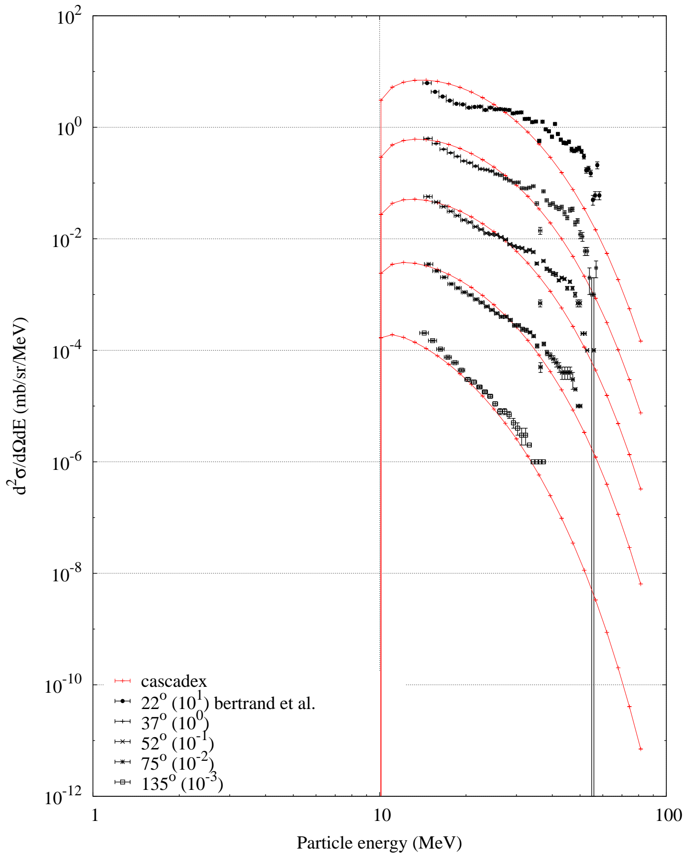
p (62 MeV) + Fe56 -- Particle spectrum
