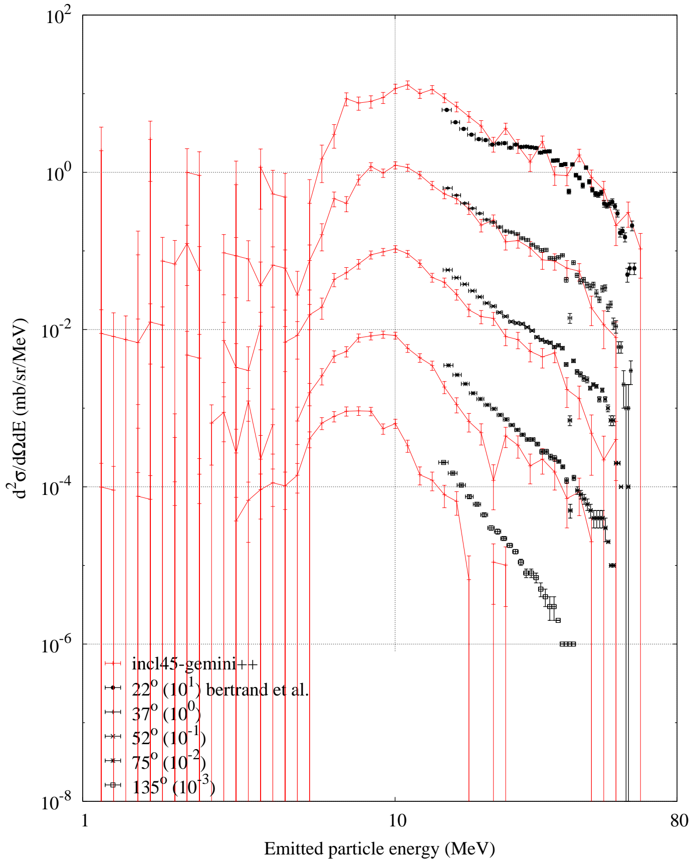
p (62 MeV) + Fe56 -- Helium-4 spectrum
