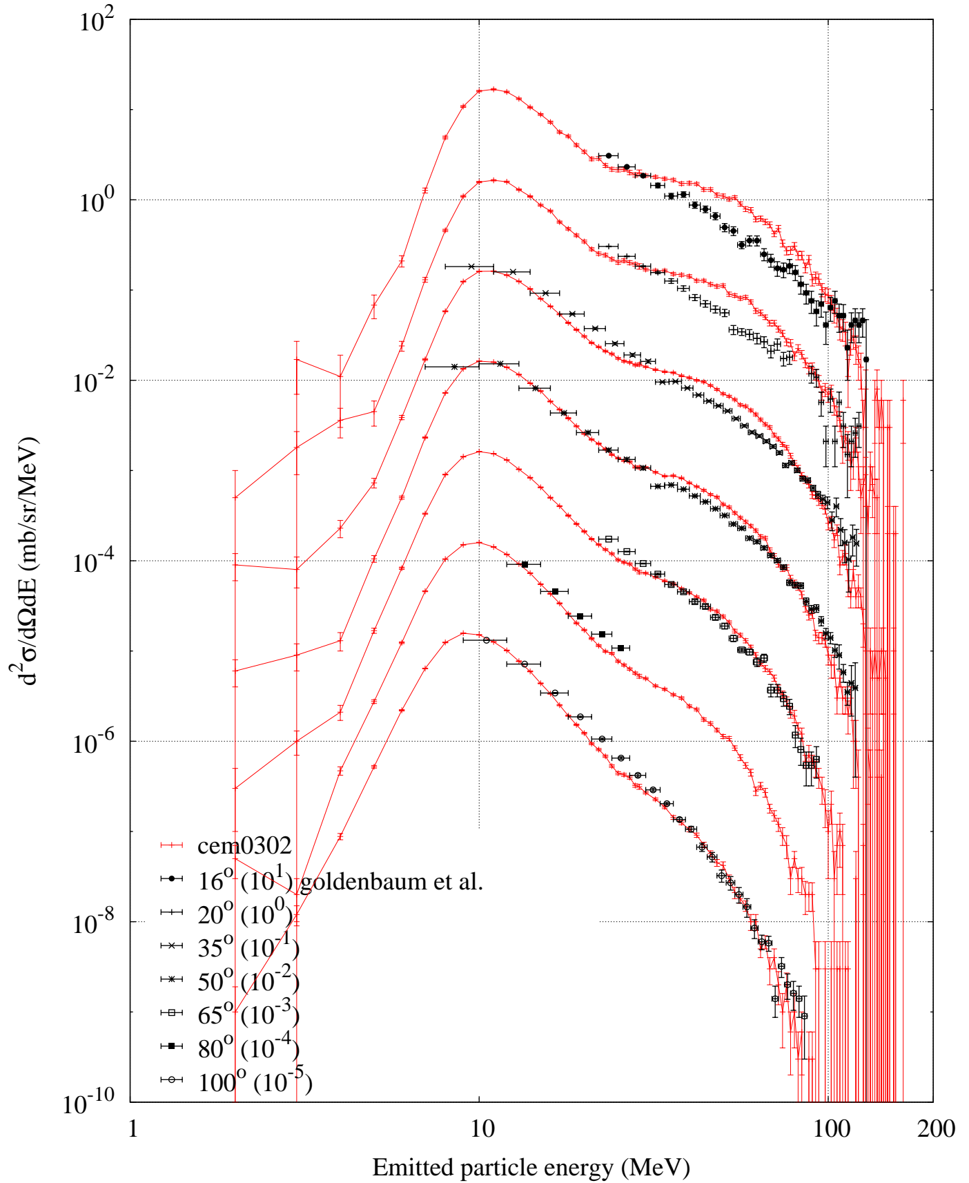
p (175 MeV) + Ni -- Helium-4 spectrum
