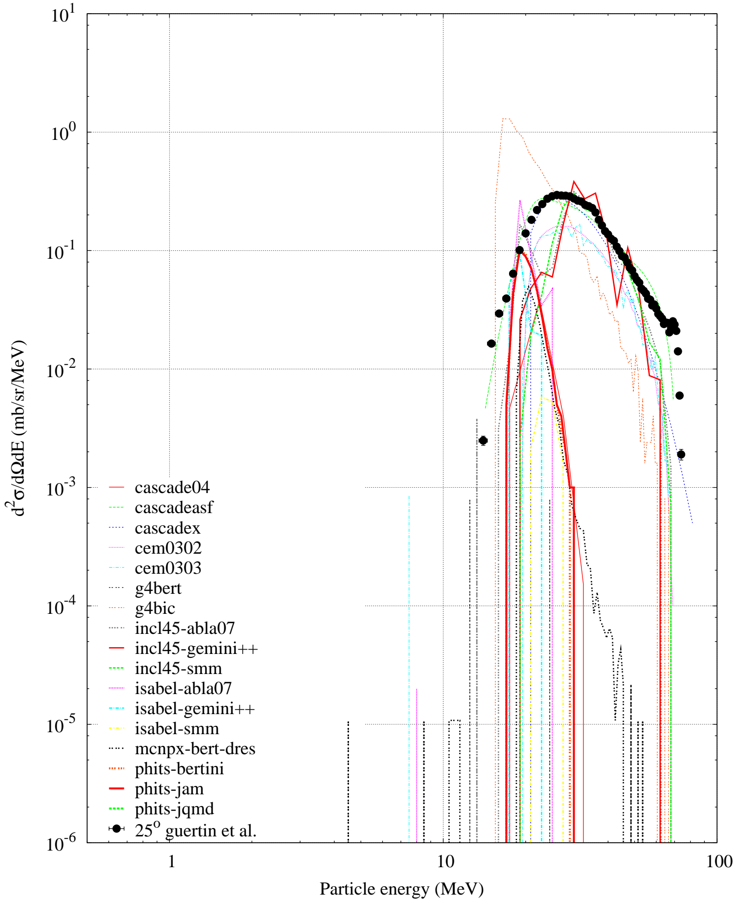
p (63 MeV) + Pb208 -- Alpha spectrum
