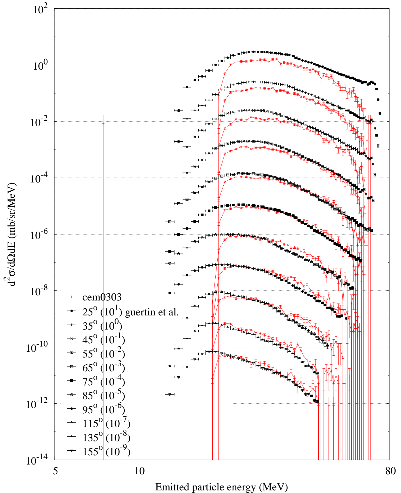
p (63 MeV) + Pb208 -- Helium-4 spectrum
