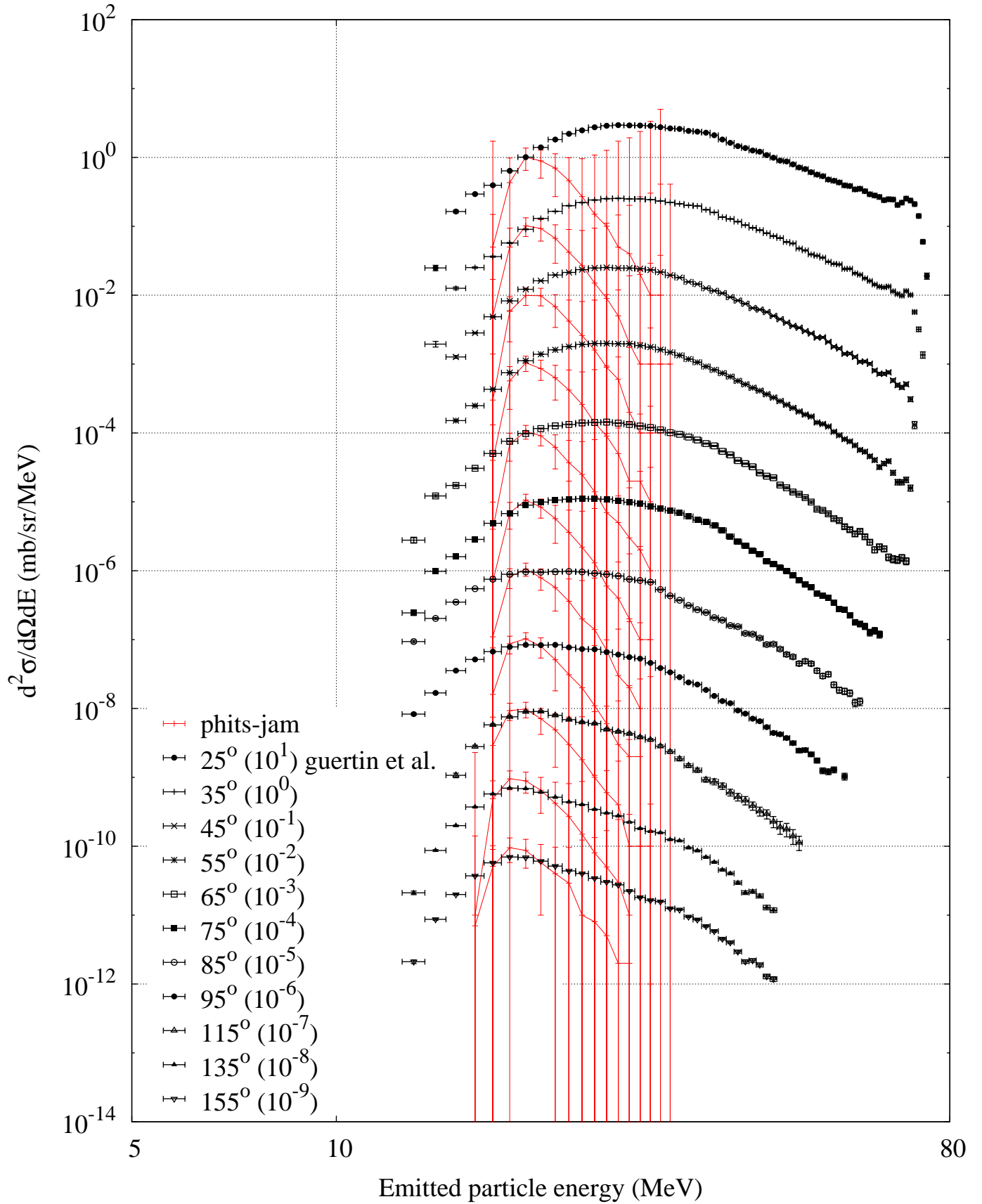
p (63 MeV) + Pb208 -- Helium-4 spectrum
