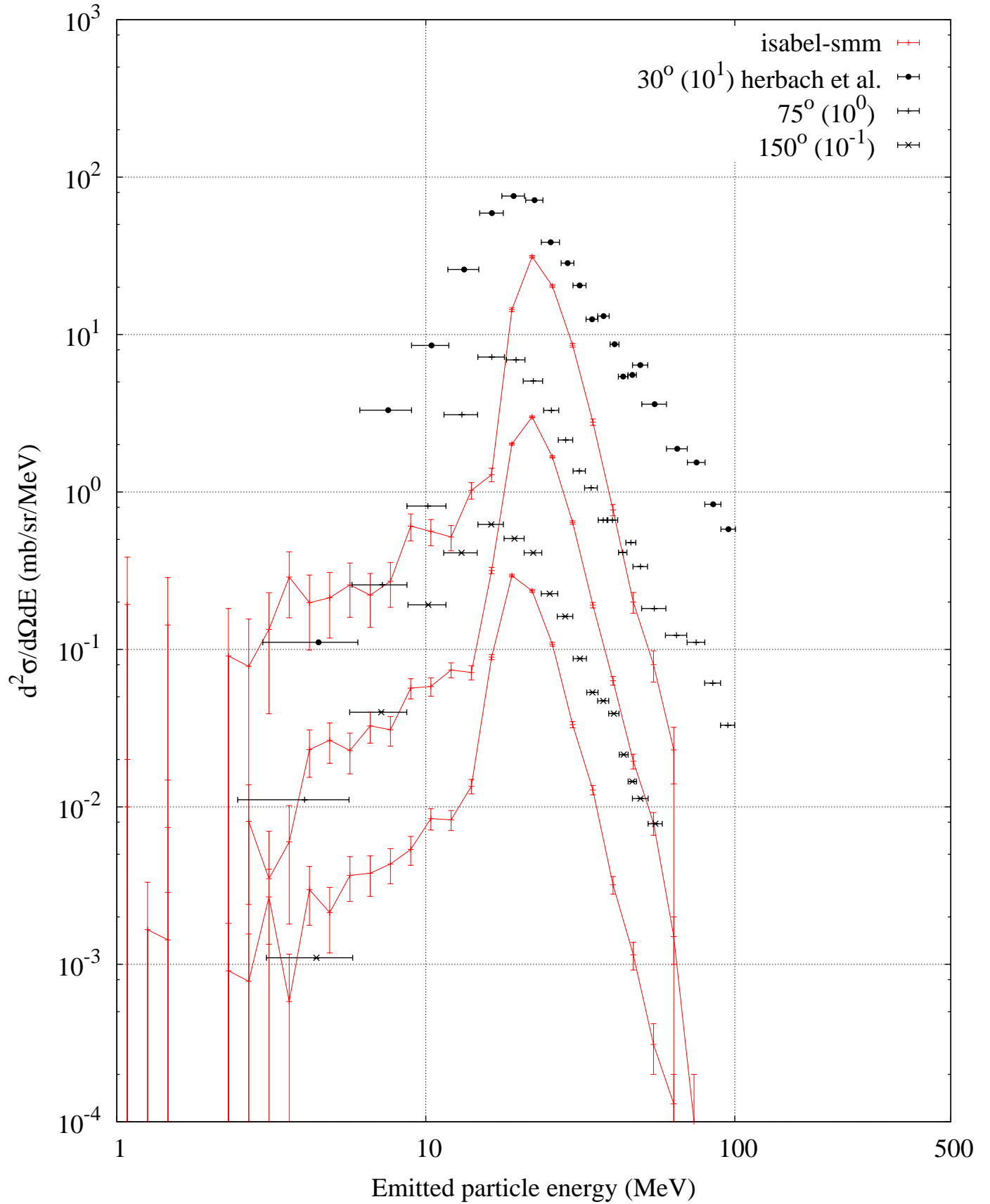
p (1200 MeV) + Ta -- Helium-4 spectrum
