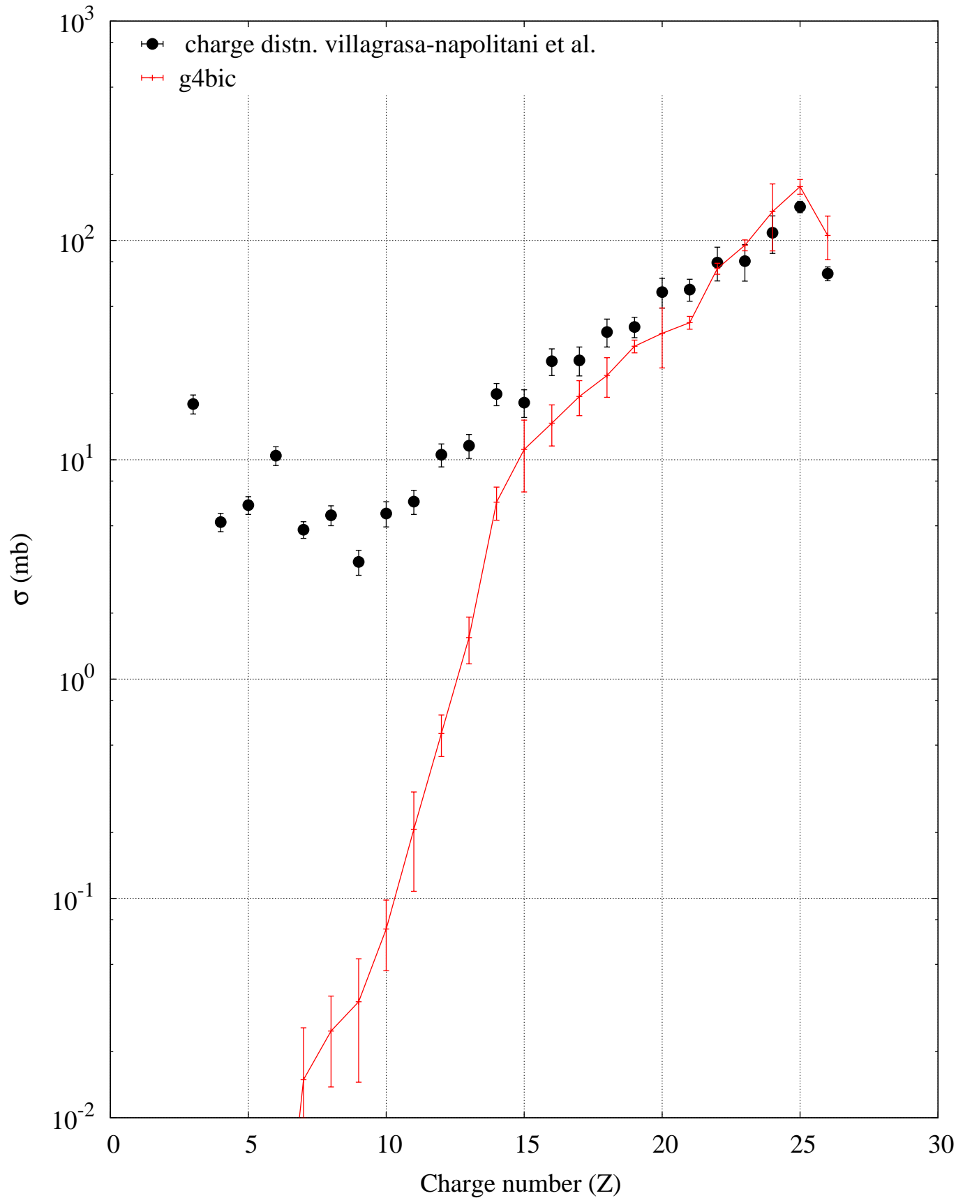
p (1000 MeV) + Fe56 -- Residue charge production
