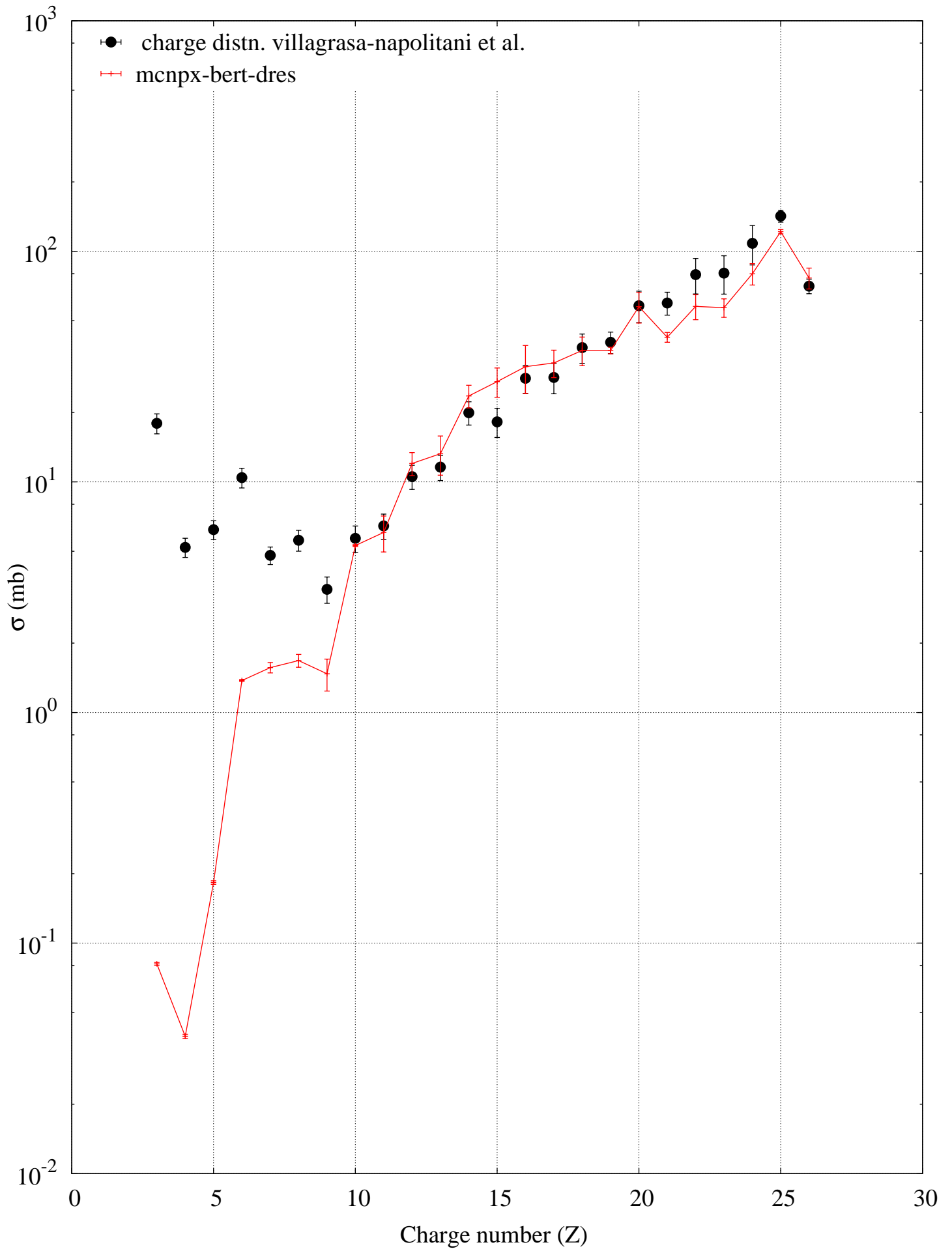
p (1000 MeV) + Fe56 -- Residue charge production
