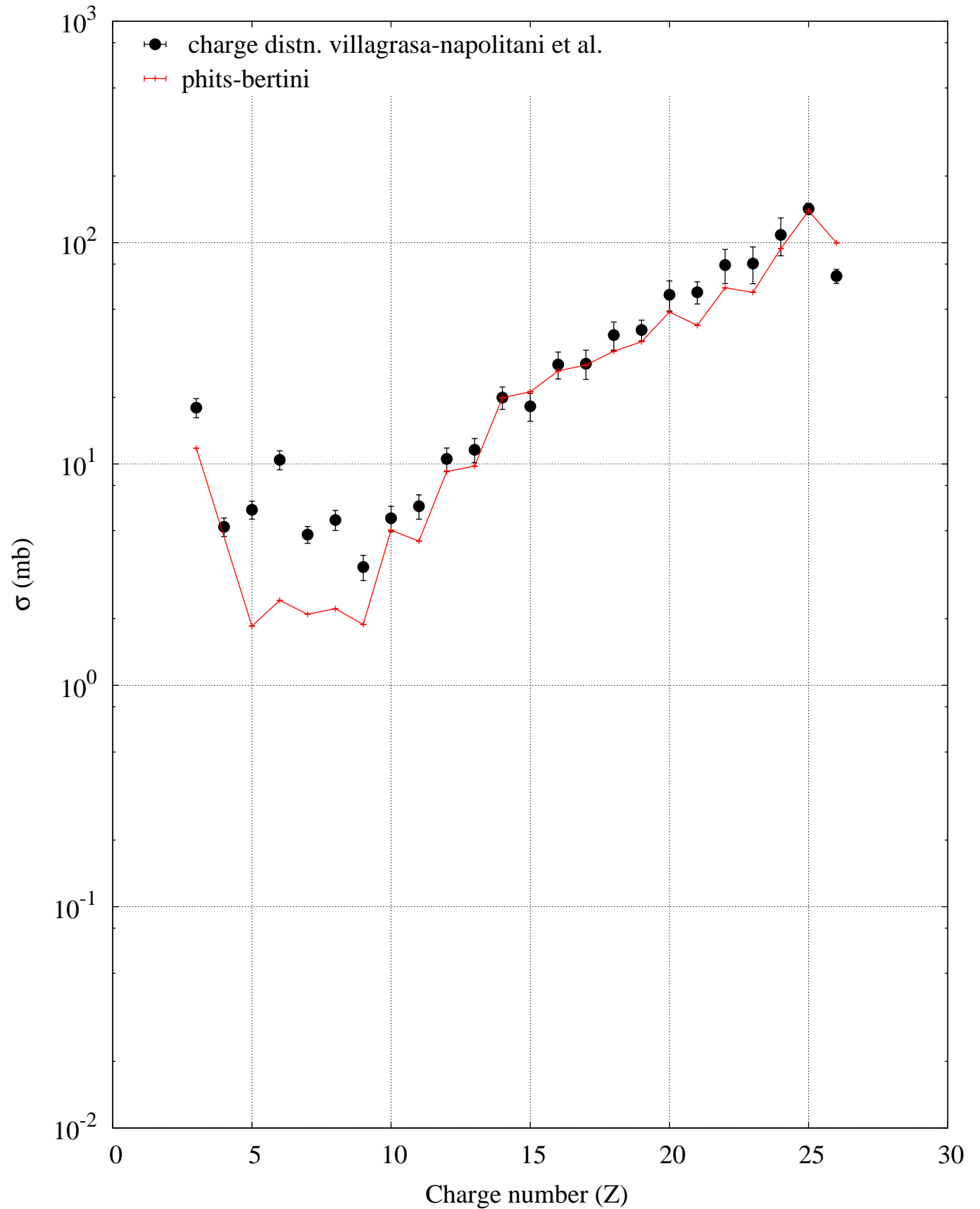
p (1000 MeV) + Fe56 -- Residue charge production
