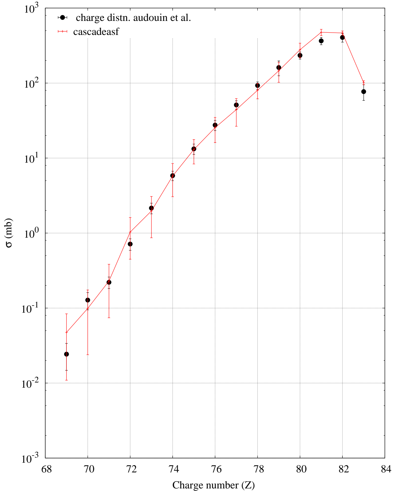
p (500 MeV) + Pb208 -- Residue charge production
