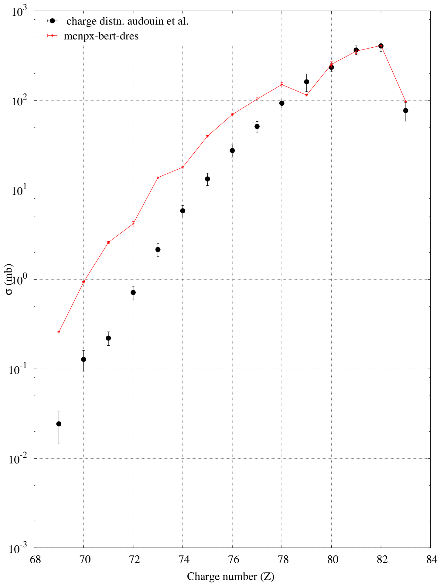
p (500 MeV) + Pb208 -- Residue charge production
