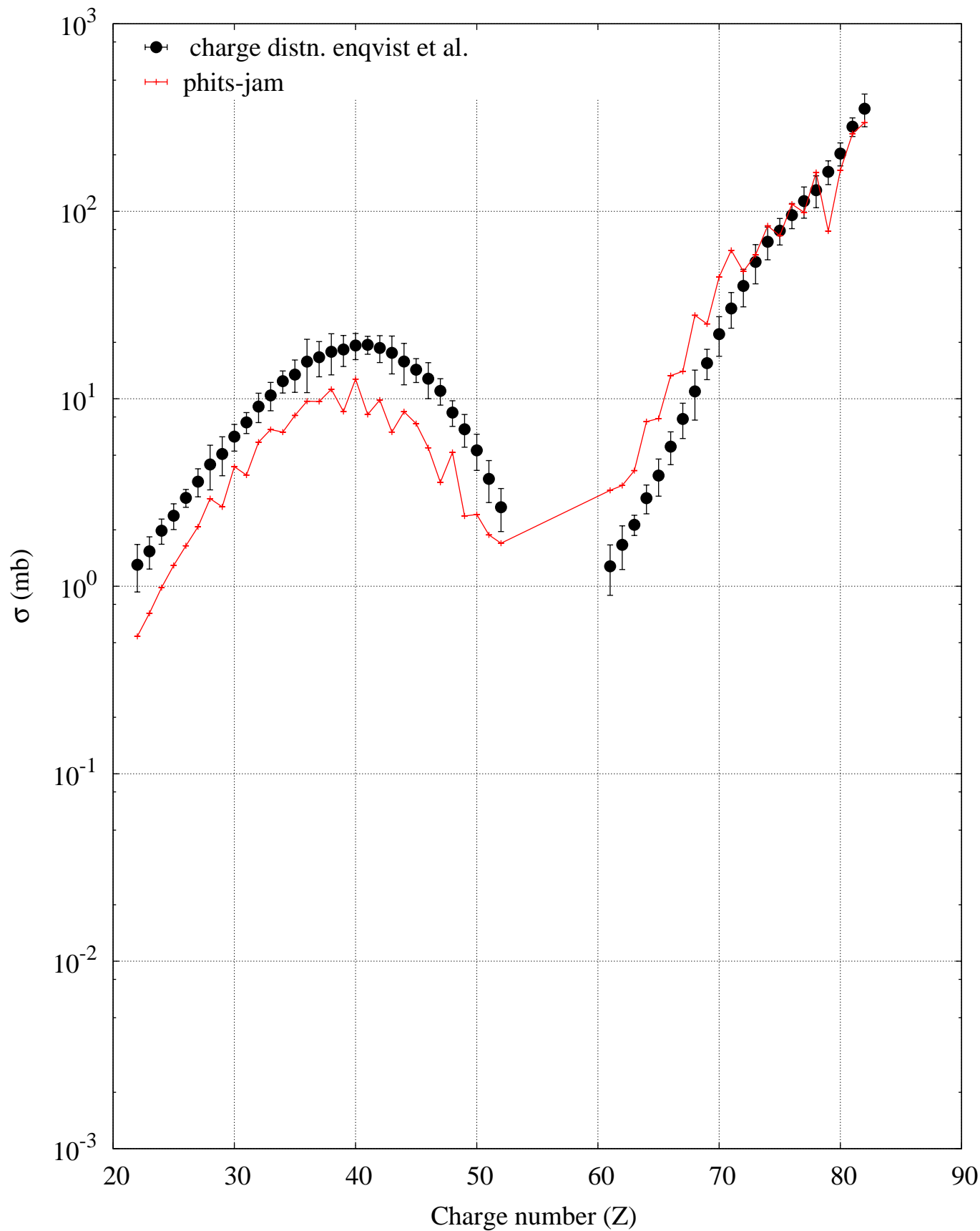
p (1000 MeV) + Pb208 -- Residue charge production
