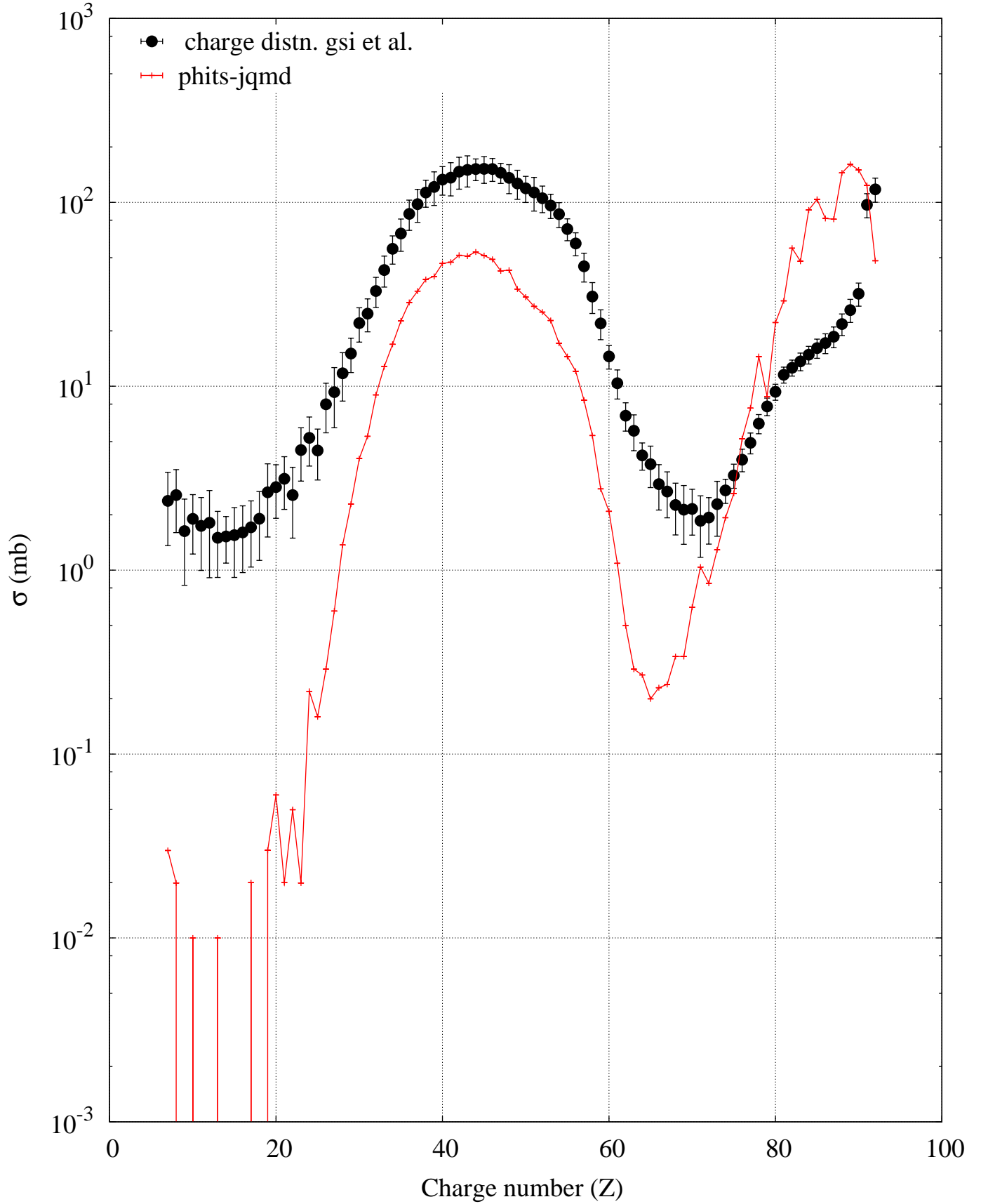
p (1000 MeV) + U238 -- Residue charge production
