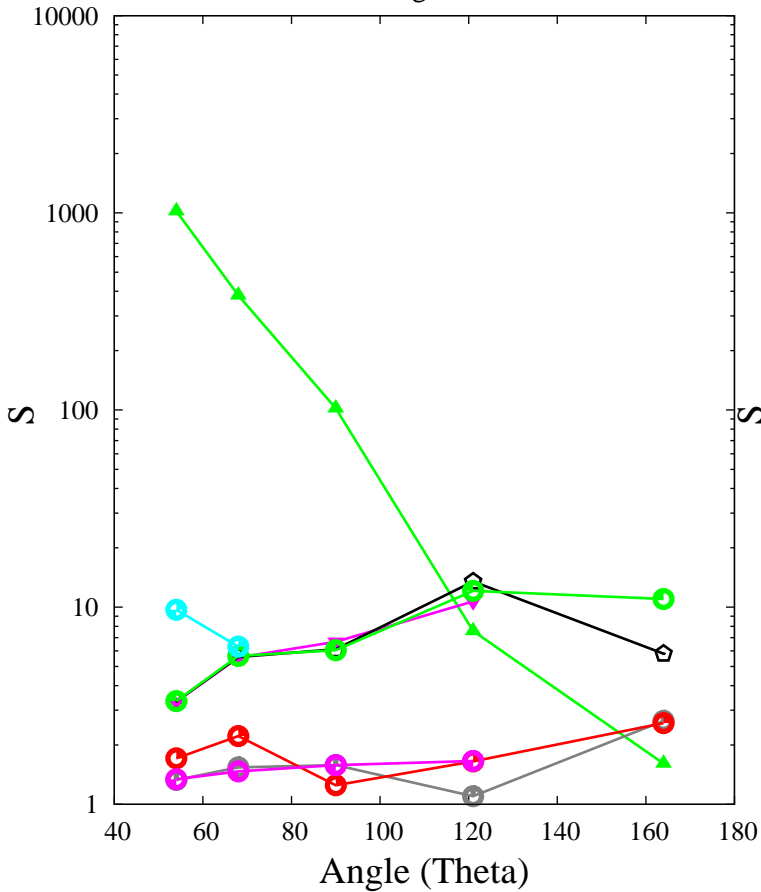
S factor - E_{\text{high}}(150+ \text{ MeV})
