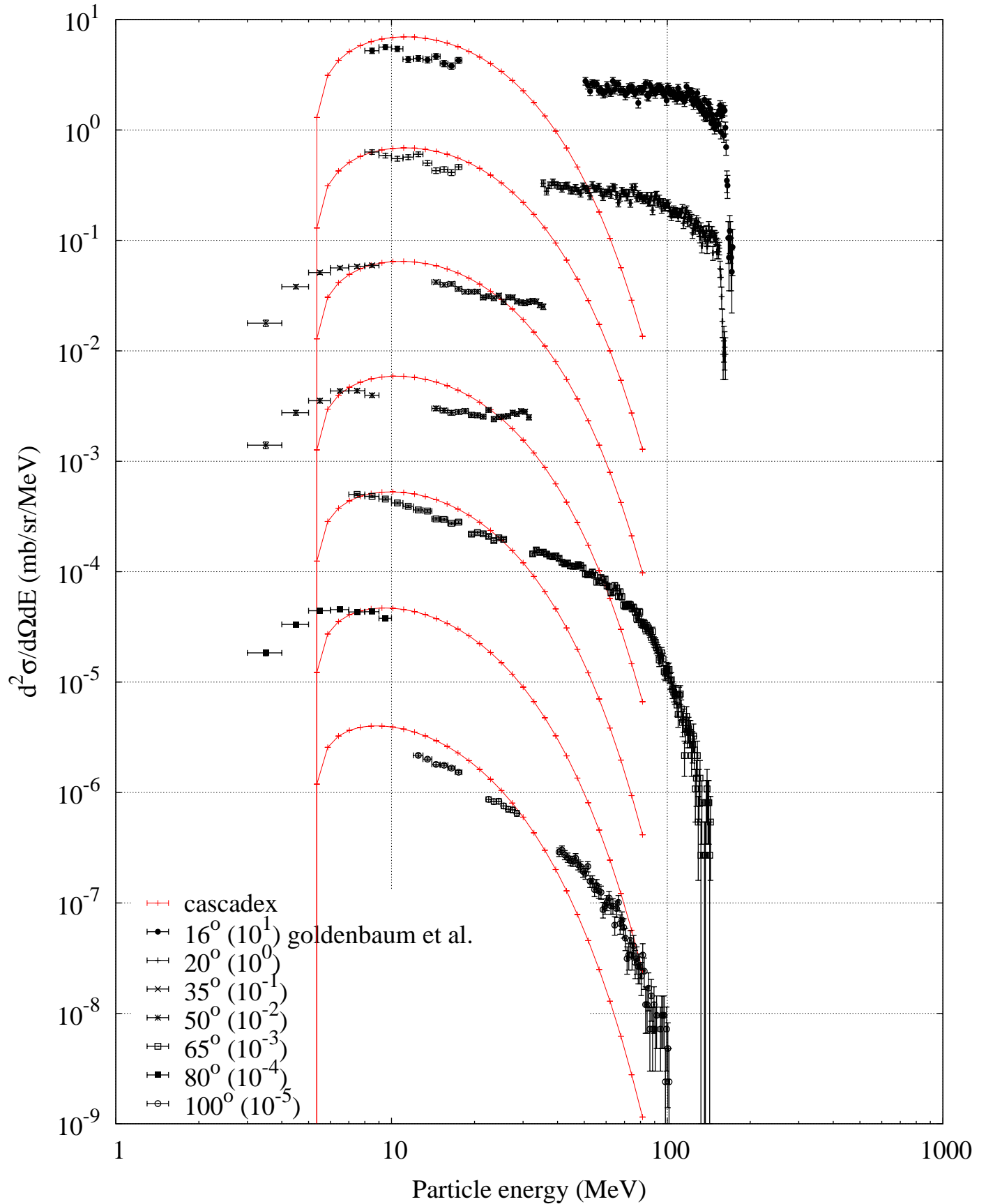
p (175 MeV) + Ni -- Particle spectrum
