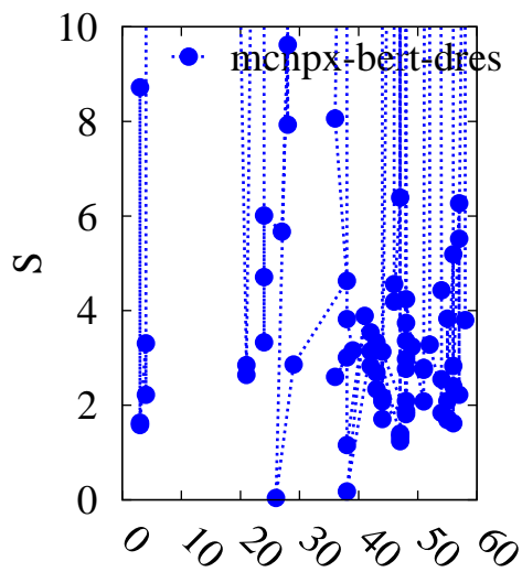
Mass number (A) S factor
