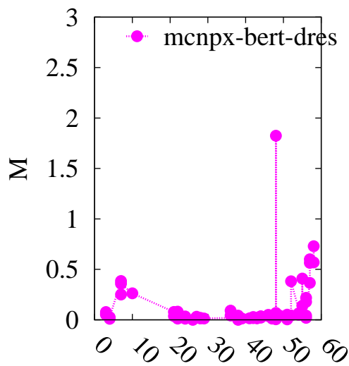
Mass number (A) M factor
