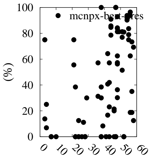
Mass number (A) P2 factor
