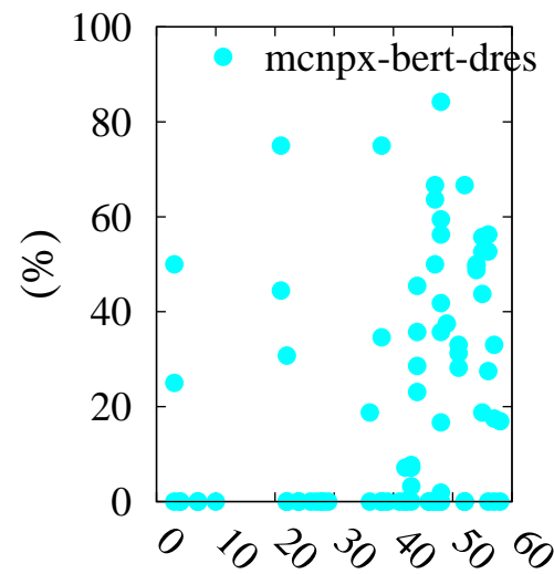
Mass number (A) P1.3 factor
