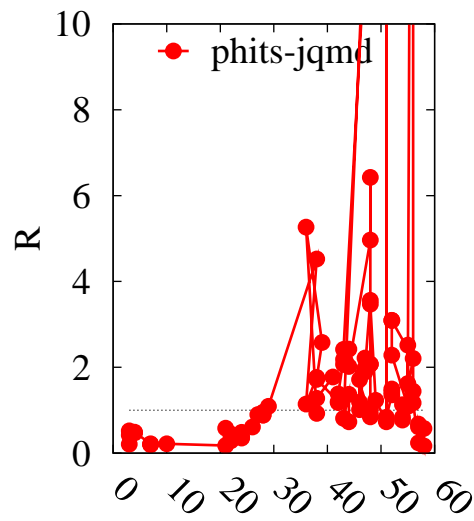
R factor
