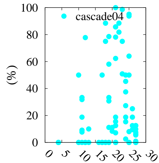
Charge number (Z) P1.3 factor
