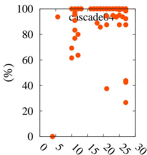
Charge number (Z) P10 factor
