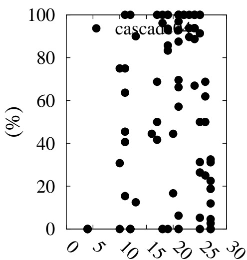
Charge number (Z) P2 factor
