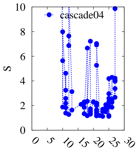
Charge number (Z) S factor
