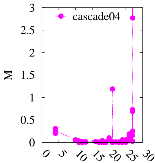
Charge number (Z) M factor
