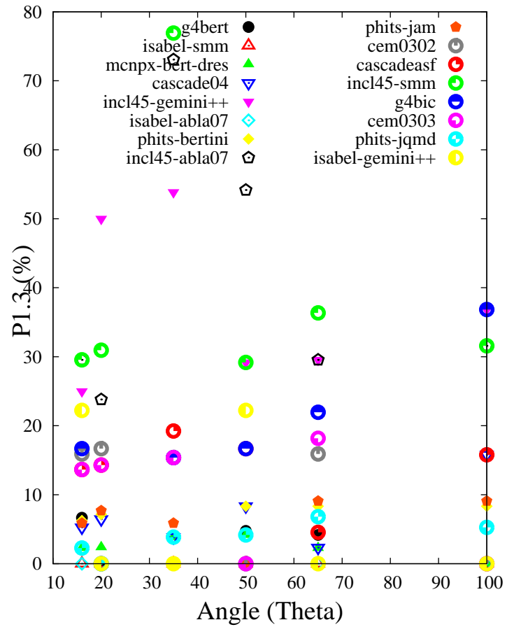
P1.3 factor - E_{\text{int}} (20-150 MeV)
