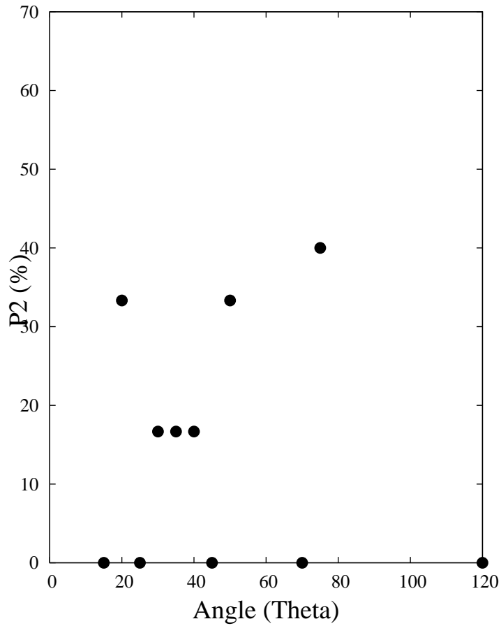
P2 factor - E_{\text{low}} (0-20 MeV)
