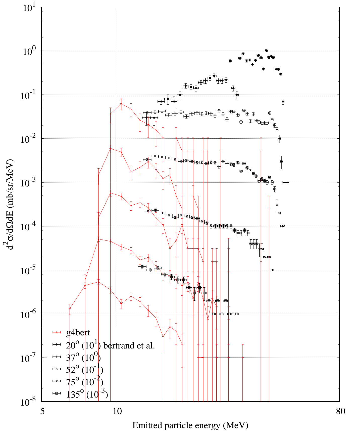
p (62 MeV) + Fe56 -- Helium-3 spectrum
