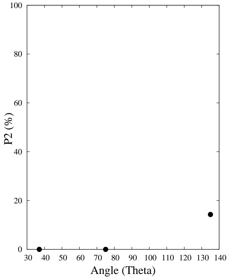
P2 factor - E_{\text{low}} (0-20 MeV)
