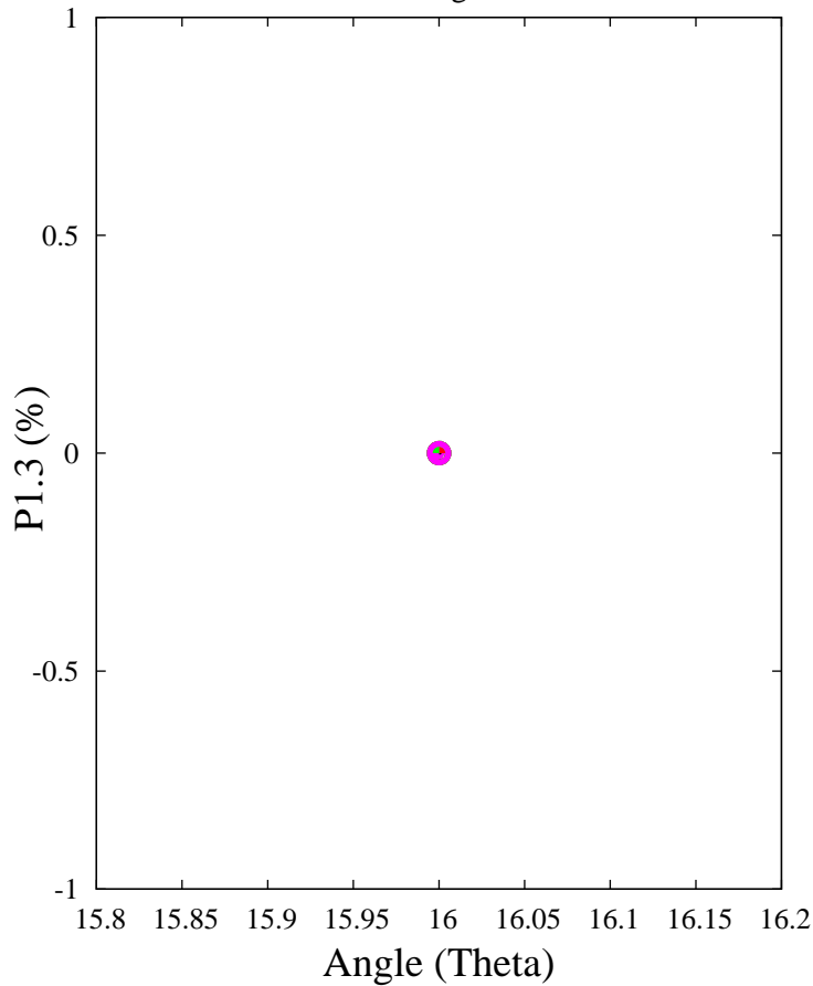
P1.3 factor - E_{\text{high}} (150+ MeV)
