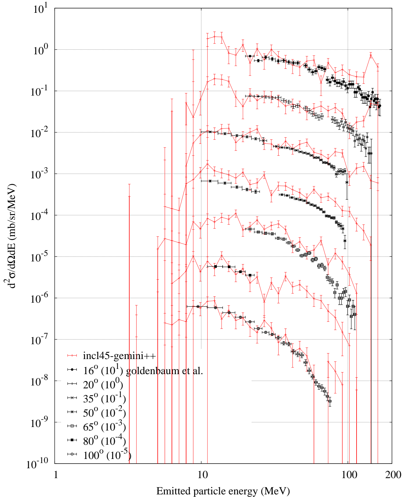
p (175 MeV) + Ni -- Helium-3 spectrum
