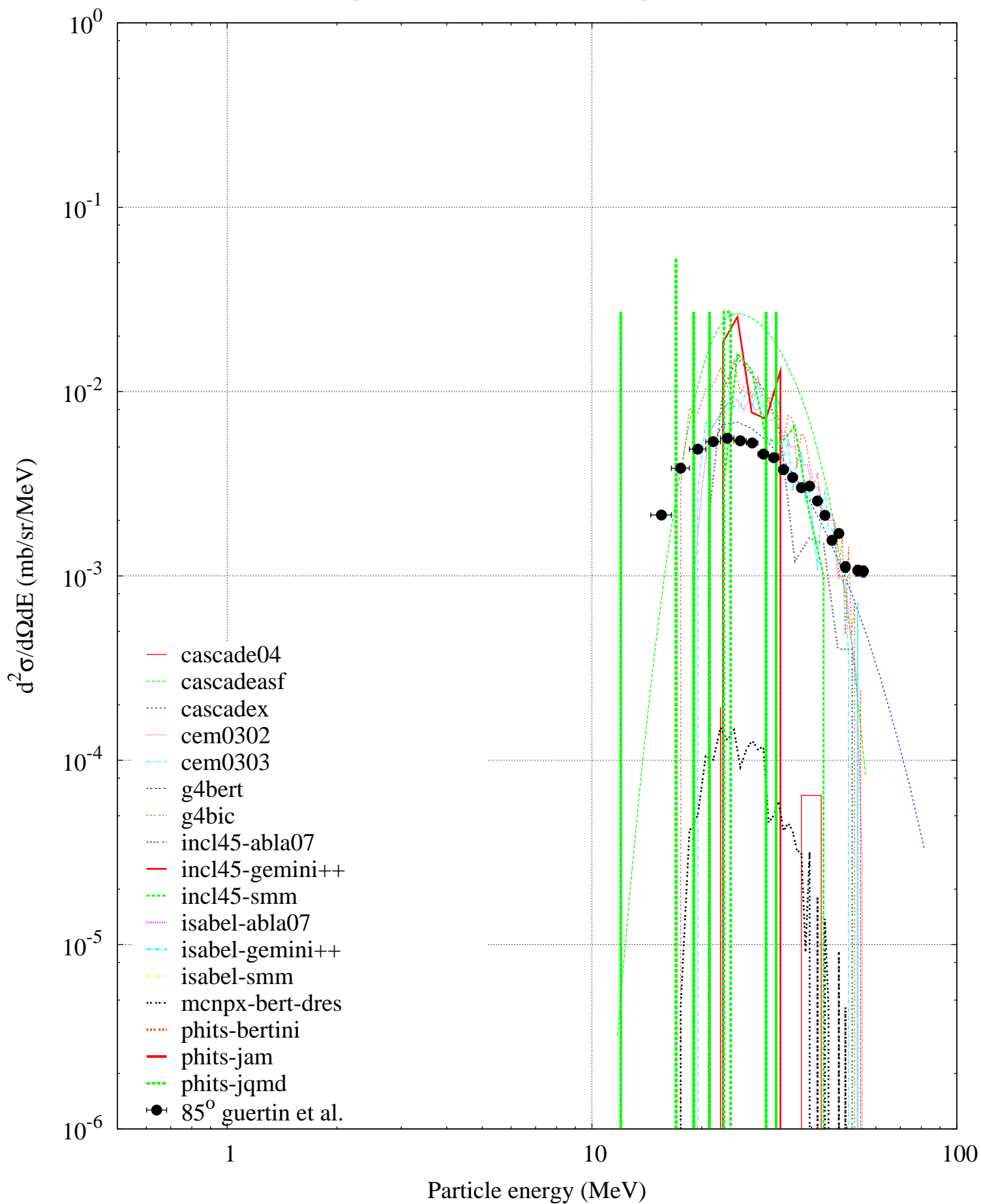
p (63 MeV) + Pb208 -- He3 spectrum
