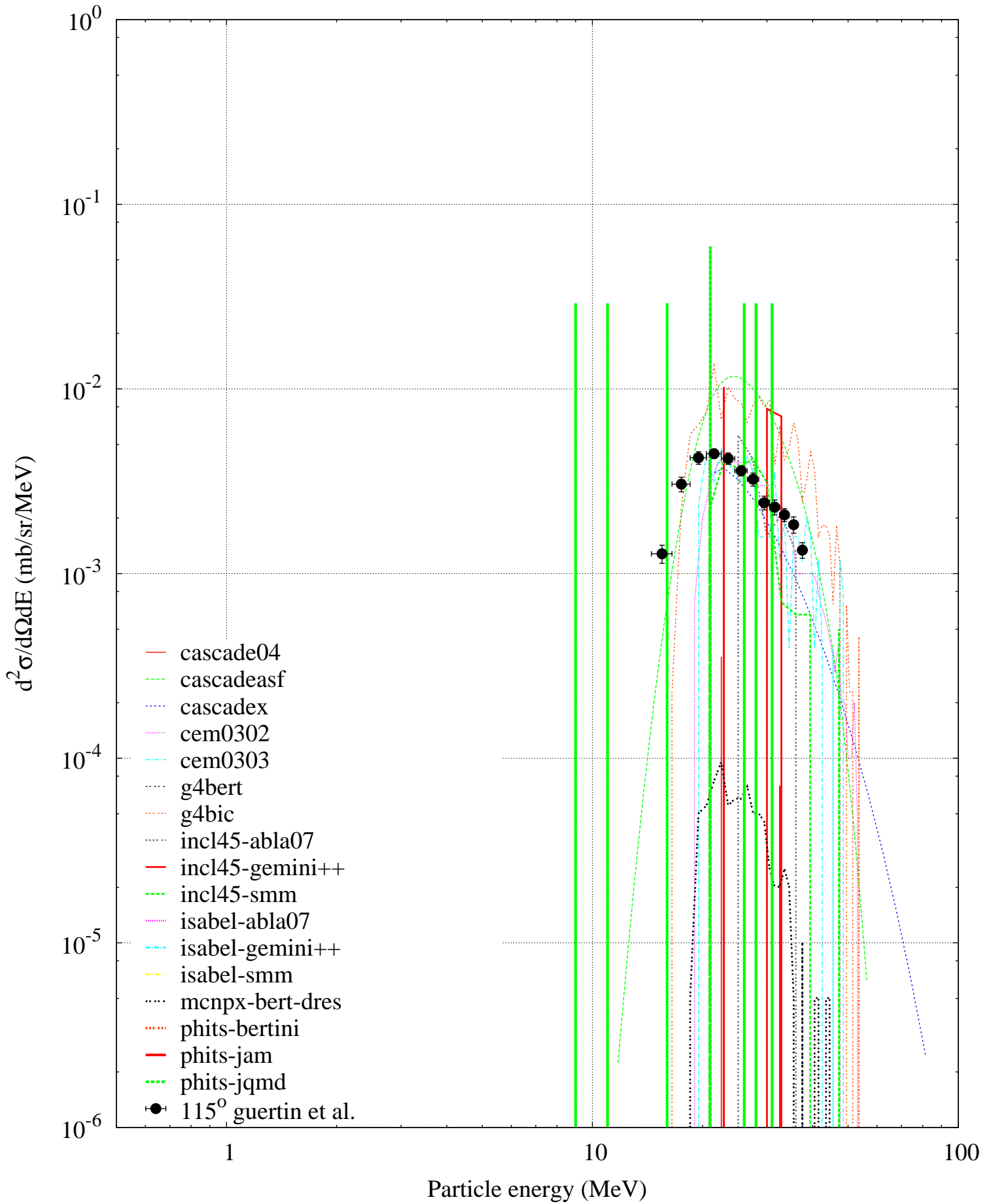
p (63 MeV) + Pb208 -- He3 spectrum
