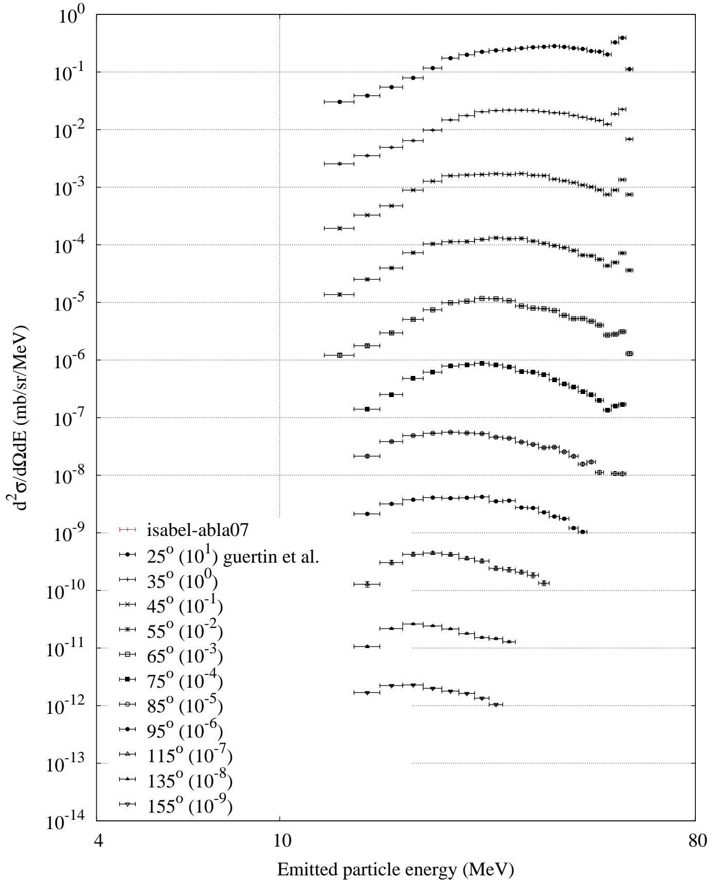
p (63 MeV) + Pb208 -- Helium-3 spectrum
