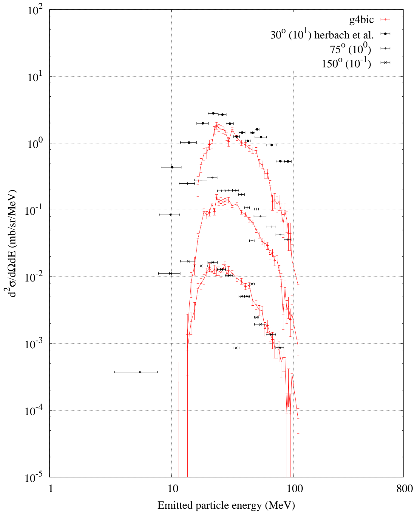
p (1200 MeV) + Ta -- Helium-3 spectrum
