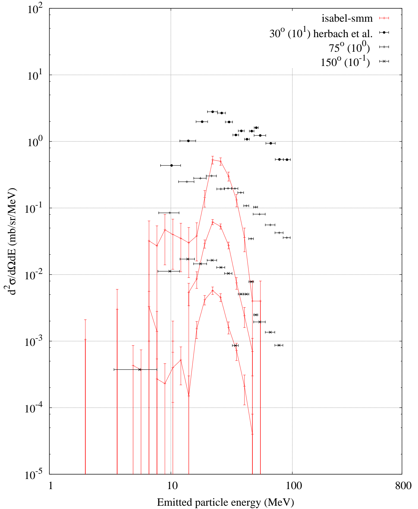
p (1200 MeV) + Ta -- Helium-3 spectrum
