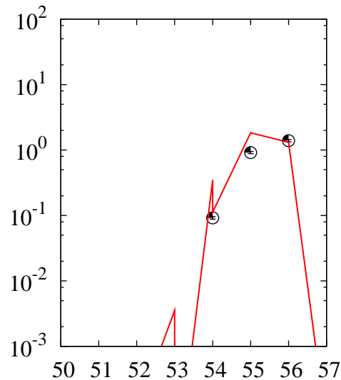
^{56}\text{Fe}(p,x)\text{Co}
