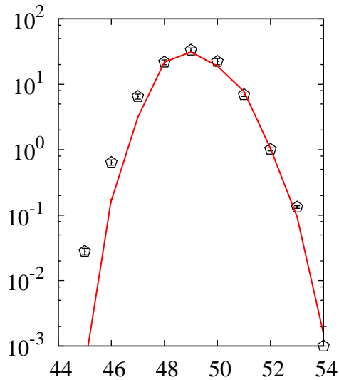
^{56}\text{Fe}(p,x)\text{V}
