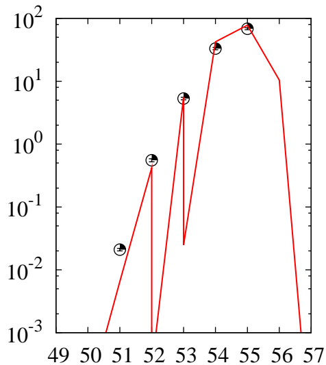
^{56}\text{Fe}(p,x)\text{Fe}
