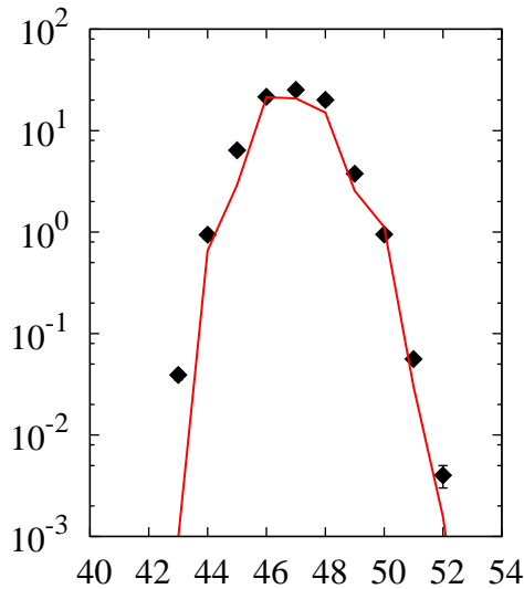
^{56}\text{Fe}(p,x)\text{Ti}
