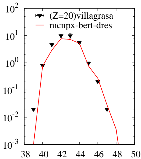
^{56}\text{Fe}(p,x)\text{Ca}
