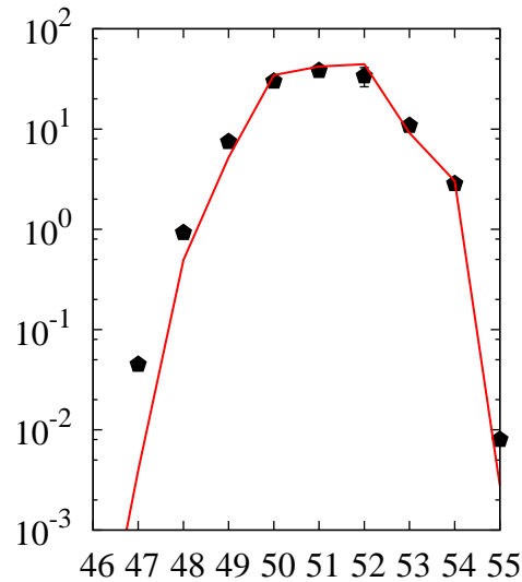
^{56}\text{Fe}(p,x)\text{Cr}
