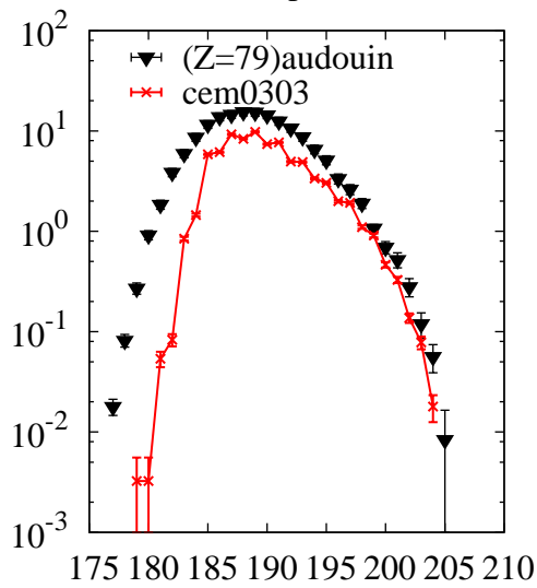
^{208}\text{Pb}(p,x)\text{Au}
