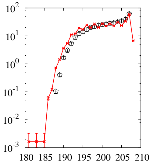
^{208}\text{Pb}(p,x)\text{Pb}
