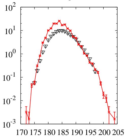
^{208}\text{Pb}(p,x)\text{Pt}
