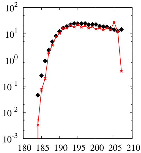
^{208}\text{Pb}(p,x)\text{Tl}
