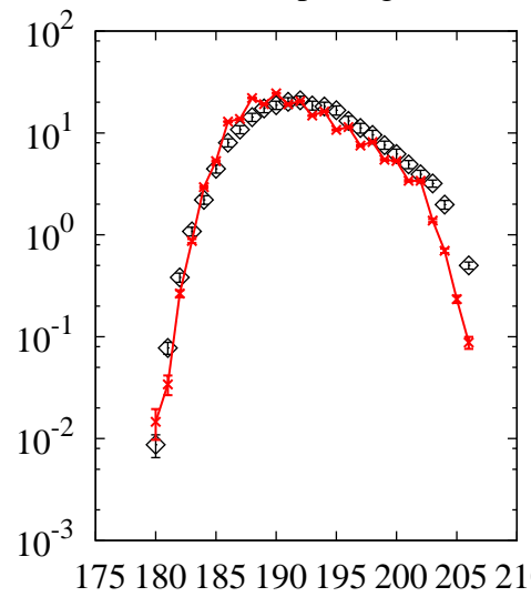
^{208}\text{Pb}(p,x)\text{Hg}
