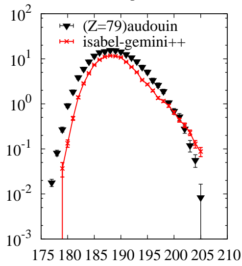
^{208}\text{Pb}(p,x)\text{Au}
