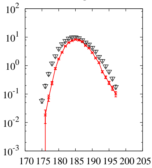
^{208}\text{Pb}(p,x)\text{Pt}
