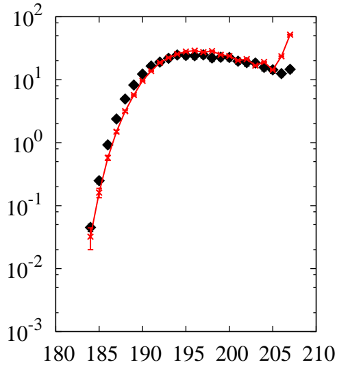
^{208}\text{Pb}(p,x)\text{Tl}
