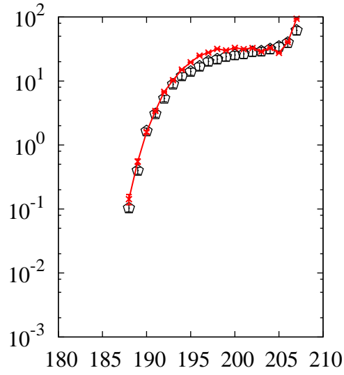
^{208}\text{Pb}(p,x)\text{Pb}
