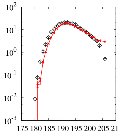
^{208}\text{Pb}(p,x)\text{Hg}
