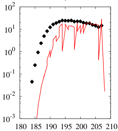
^{208}\text{Pb}(p,x)\text{Tl}
