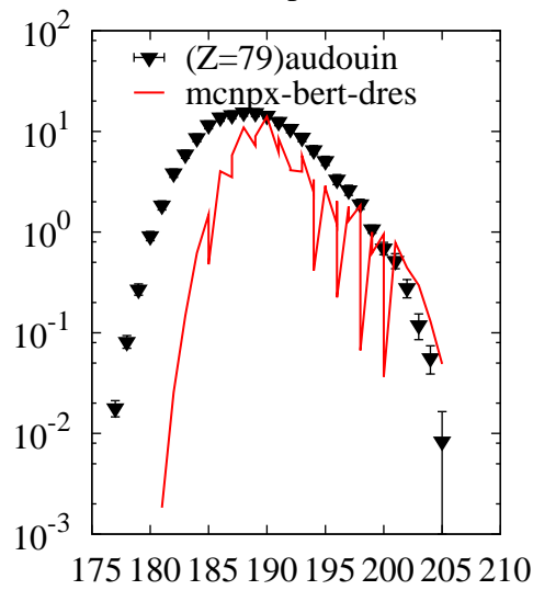
^{208}\text{Pb}(p,x)\text{Au}
