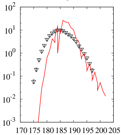
^{208}\text{Pb}(p,x)\text{Pt}
