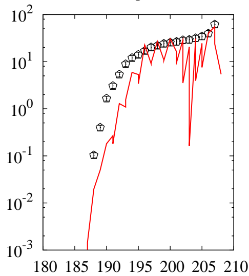
^{208}\text{Pb}(p,x)\text{Pb}
