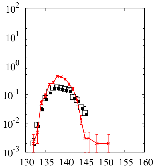
^{208}\text{Pb}(p,x)\text{Pm}
