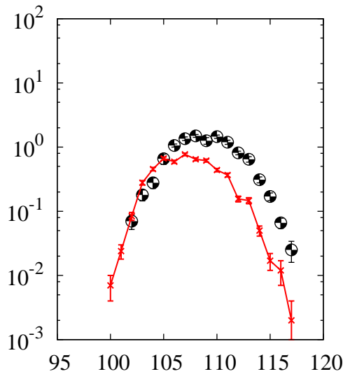
^{208}\text{Pb}(p,x)\text{Ag}
