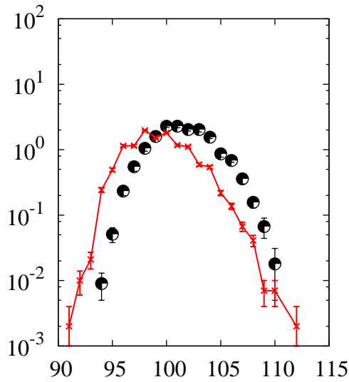
^{208}\text{Pb}(p,x)\text{Ru}
