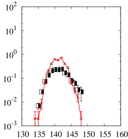
^{208}\text{Pb}(p,x)\text{Sm}
