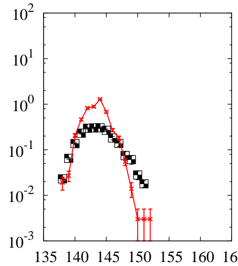
^{208}\text{Pb}(p,x)\text{Eu}
