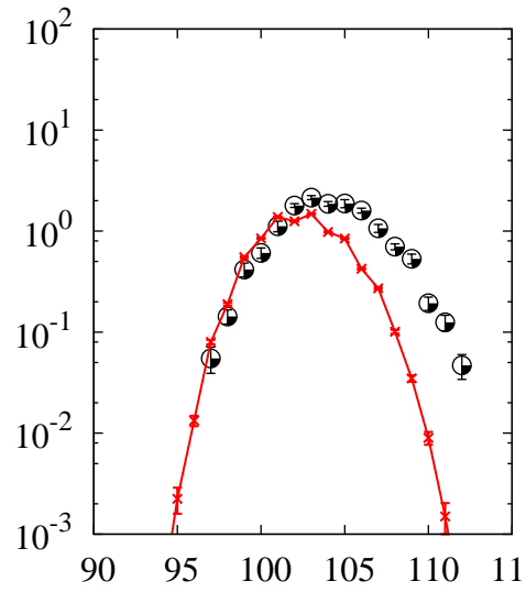
^{208}\text{Pb}(p,x)\text{Rh}
