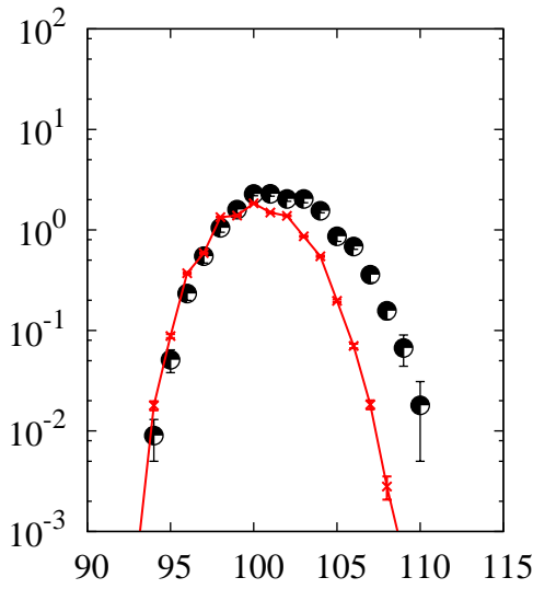
^{208}\text{Pb}(p,x)\text{Ru}
