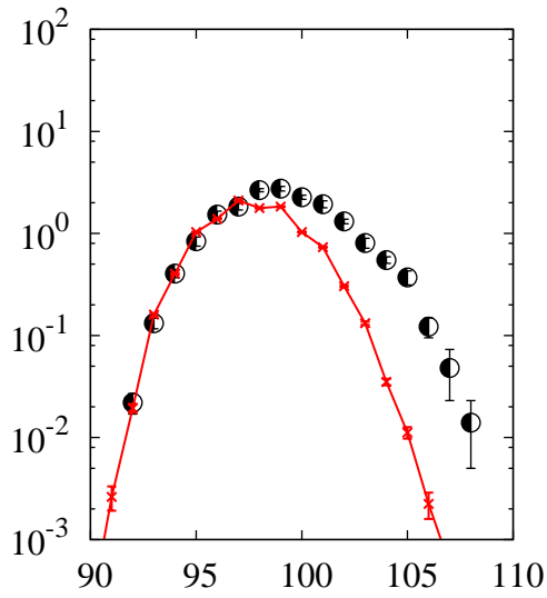
^{208}\text{Pb}(p,x)\text{Tc}
