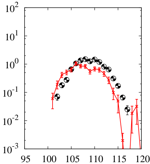
^{208}\text{Pb}(p,x)\text{Ag}
