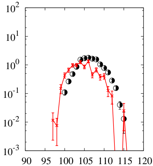
^{208}\text{Pb}(p,x)\text{Pd}
