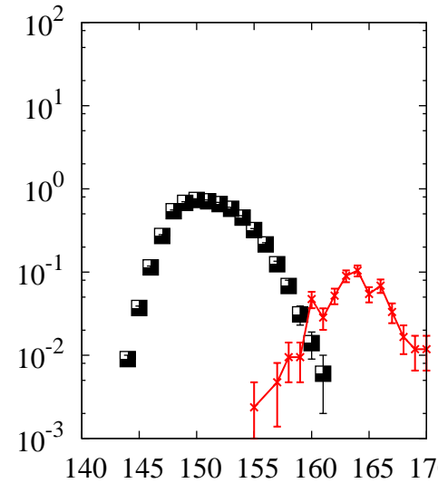
^{208}\text{Pb}(p,x)\text{Dy}
