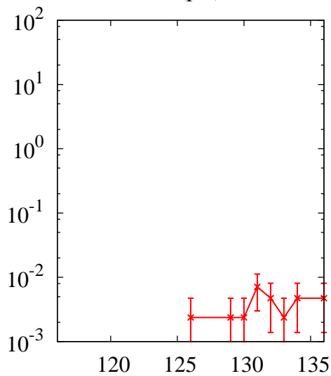
^{208}\text{Pb}(p,x)\text{Ba}
