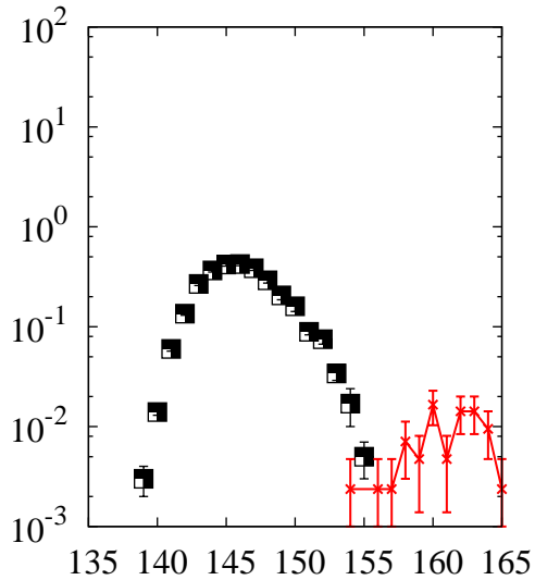
^{208}\text{Pb}(p,x)\text{Gd}
