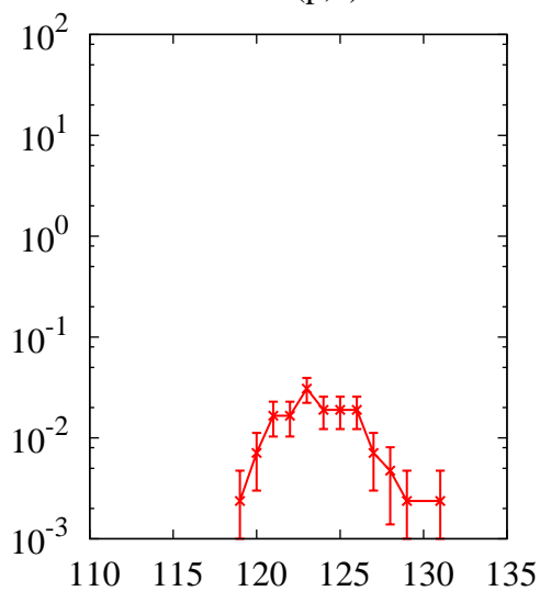
^{208}\text{Pb}(p,x)\text{I}
