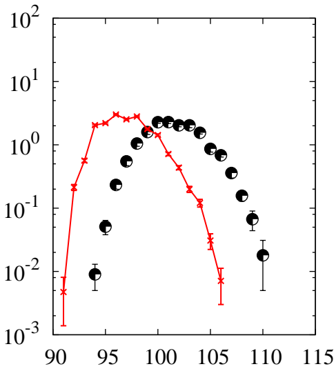
^{208}\text{Pb}(p,x)\text{Ru}
