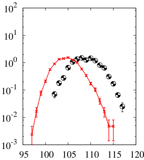
^{208}\text{Pb}(p,x)\text{Ag}
