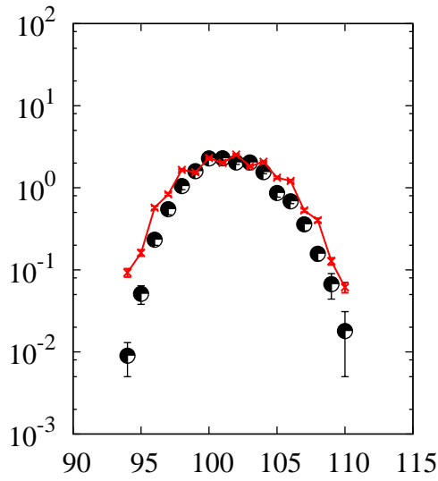
^{208}\text{Pb}(p,x)\text{Ru}
