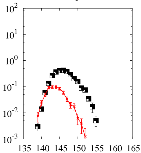
^{208}\text{Pb}(p,x)\text{Gd}
