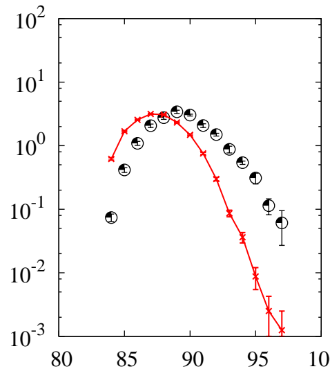
^{208}\text{Pb}(p,x)\text{Y}
