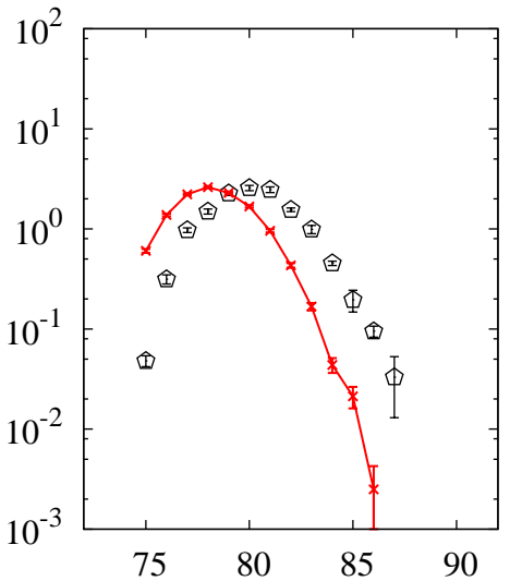
^{208}\text{Pb}(p,x)\text{Br}
