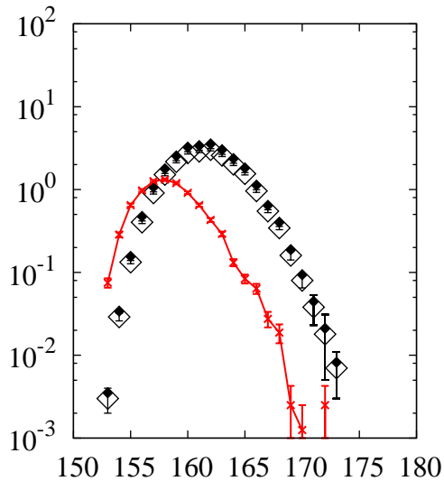
^{208}\text{Pb}(p,x)\text{Yb}
