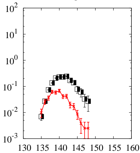
^{208}\text{Pb}(p,x)\text{Sm}
