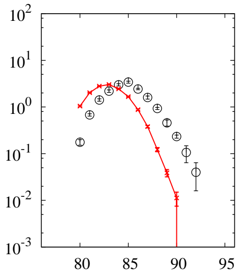
^{208}\text{Pb}(p,x)\text{Rb}
