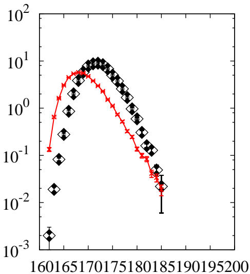
^{208}\text{Pb}(p,x)\text{W}
