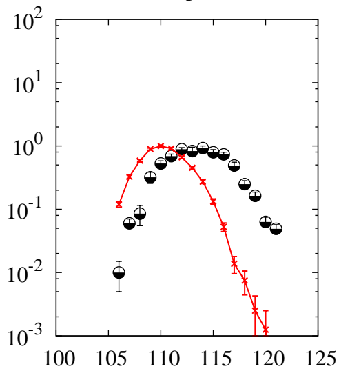
^{208}\text{Pb}(p,x)\text{In}
