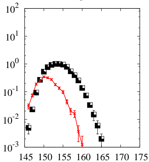
^{208}\text{Pb}(p,x)\text{Ho}
