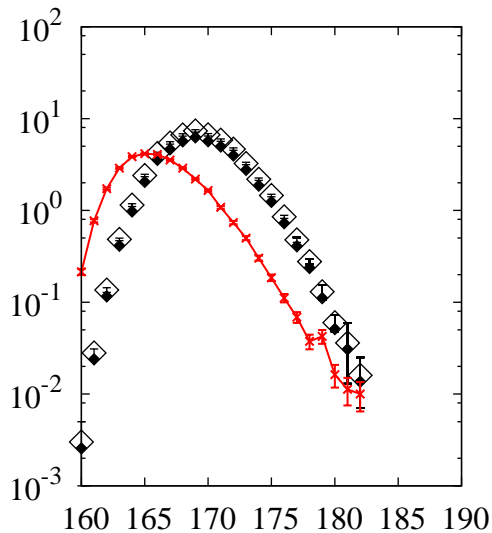
^{208}\text{Pb}(p,x)\text{Ta}
