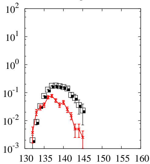
^{208}\text{Pb}(p,x)\text{Pm}
